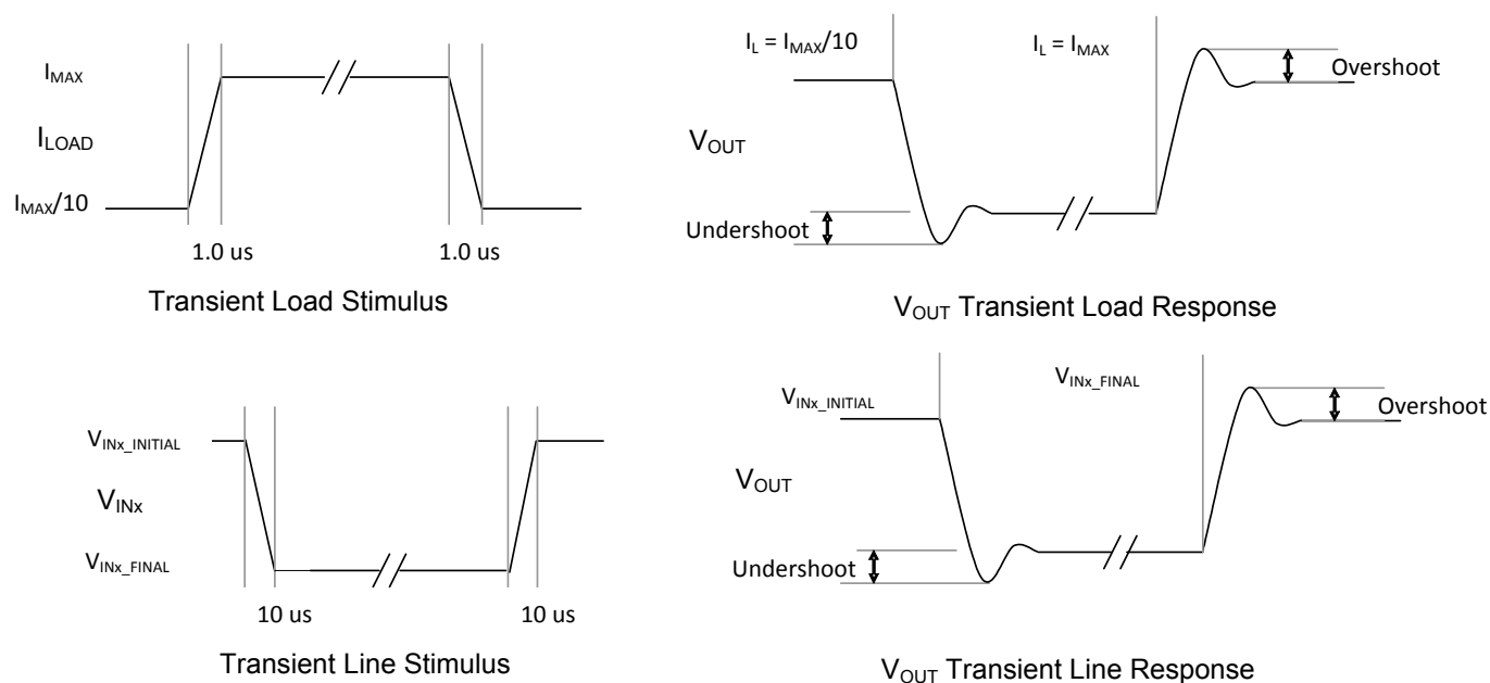
Figure 25. Transient waveforms
