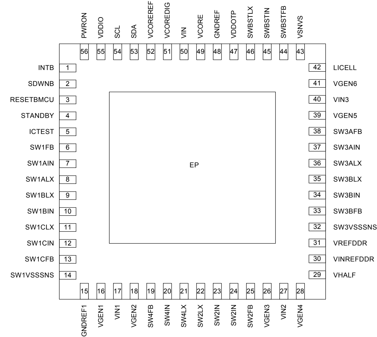
Figure 3. Pinout diagram
